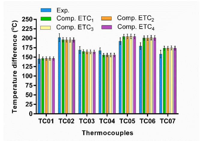
Fig. 15. 20RR sample in the 20030 test condition: comparison of the tube wall temperature increase obtained with the experiments and CFD simulations, using different RR thermal conductivities [ ETC_1 = 500 W/mK, ETC_2 = 1500 W/mK, ETC_3 = 2500 W/mK, and ETC_4 = 3500 W/mK]. The computed values were obtained using the k-\omega SST turbulence model.
