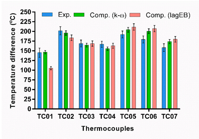
Fig. 13. 20RR sample in the 20030 test condition: comparison of the tube wall temperature increase obtained with the experiments and CFD simulations, using two different turbulence models.
