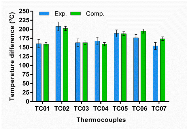
Fig. 17. Comparison of the tube wall temperature increase obtained with the experiments and CFD simulations, using the k-\omega SST turbulence model for the 40RR sample at 20030 test condition.
