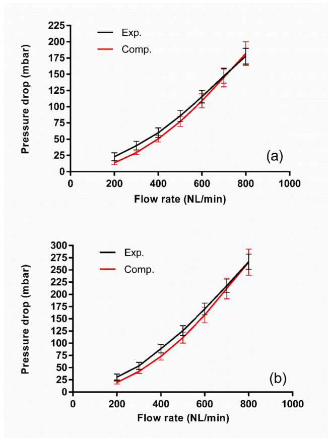
Fig. 10. Validation of the experimental pressure drop data against the numerical models; (a) 20RR sample, (b) 40RR sample.
