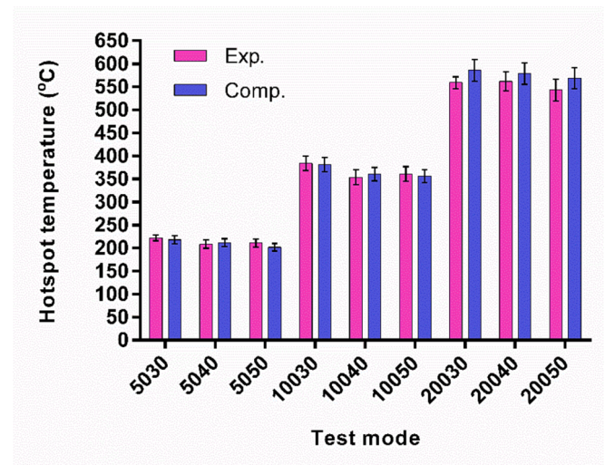
Fig. 12. SP sample: validation of the numerical study against the experimental test data in terms of hotspot temperatures. The computed values were obtained using the k-\omega SST turbulence model.
