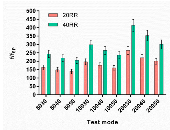
Fig. 22. The comparison of growth in the friction factors produced by the RR inserts corresponding to the SP absorber ( f/f_{sp} ) for various test conditions.
